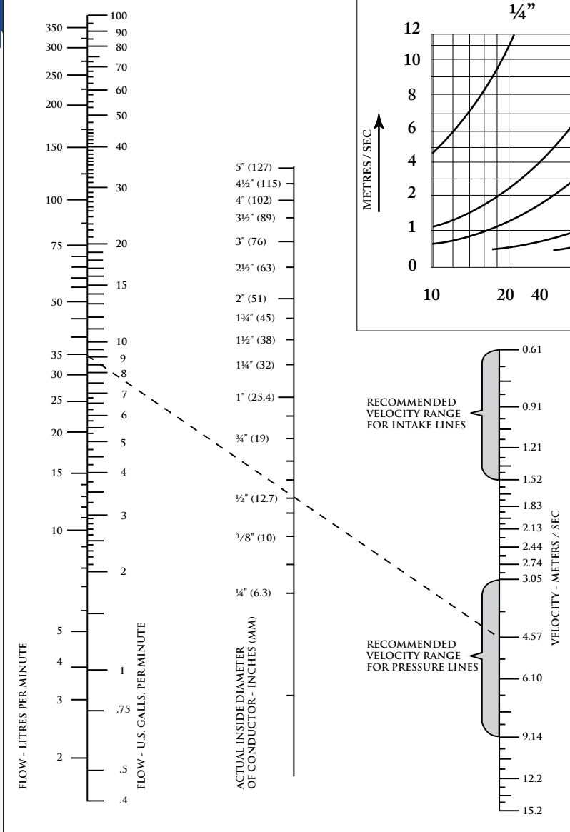
Fig.1 Flow Nomograph
