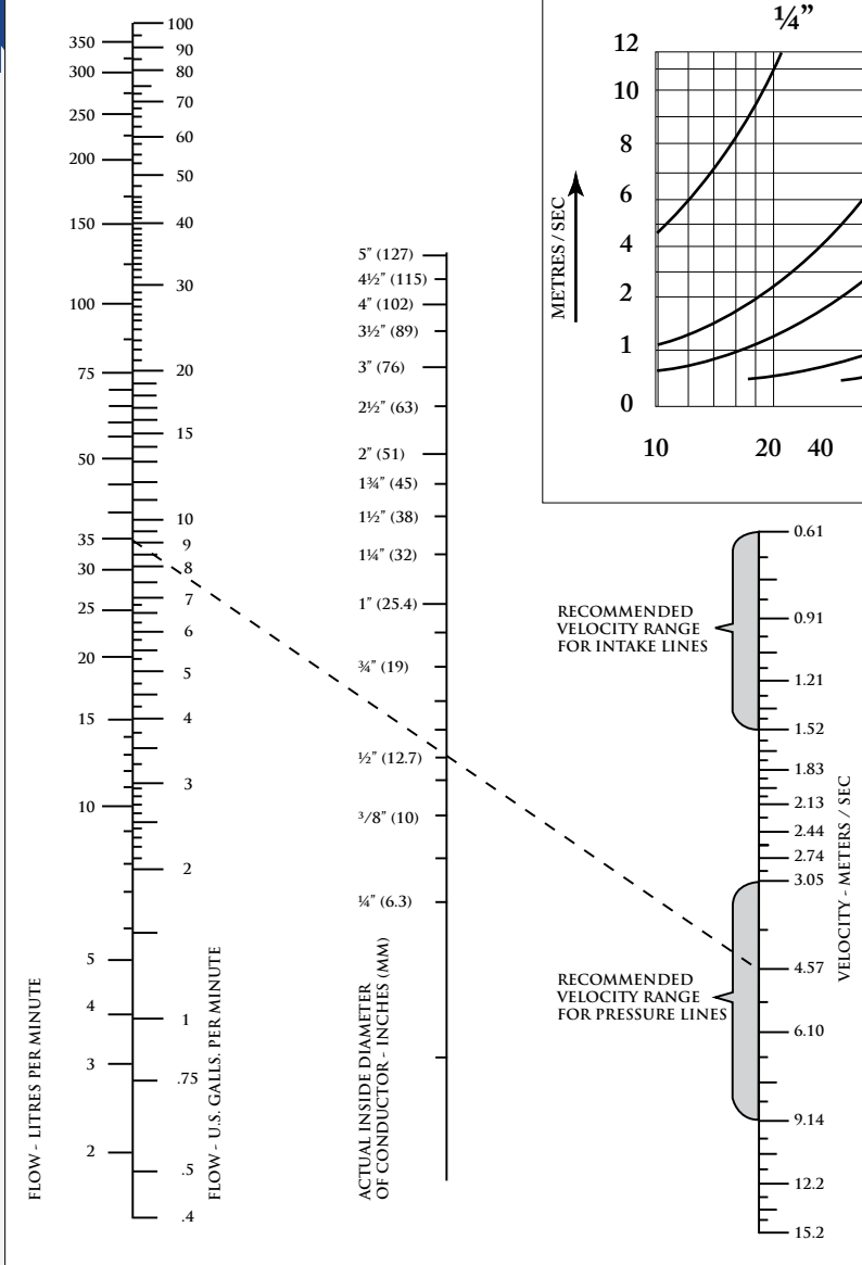
Fig.1 Flow Nomograph
